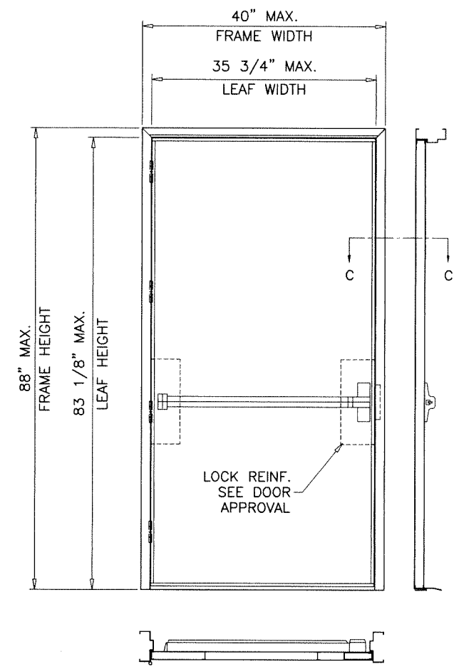
OUTSWING SINGLE STEEL DOOR
