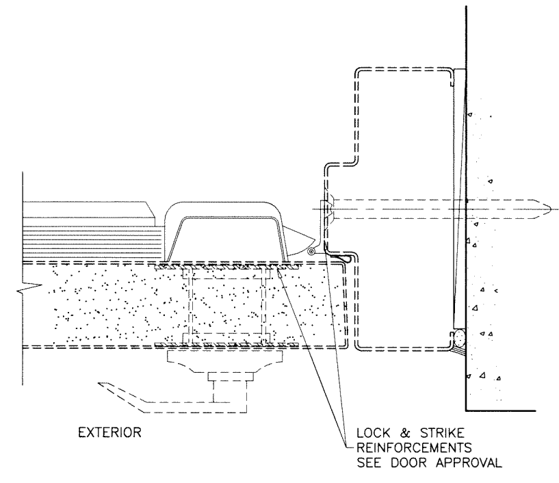
SECTION C-C '6200' SERIES RIM EXIT DEVICE
