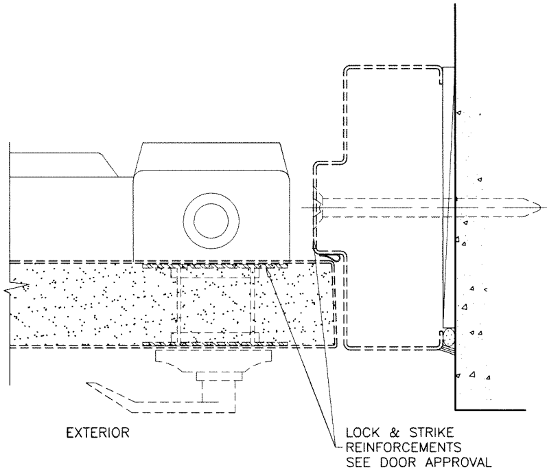
SECTION E-E '6200' SERIES SVR EXIT DEVICE
