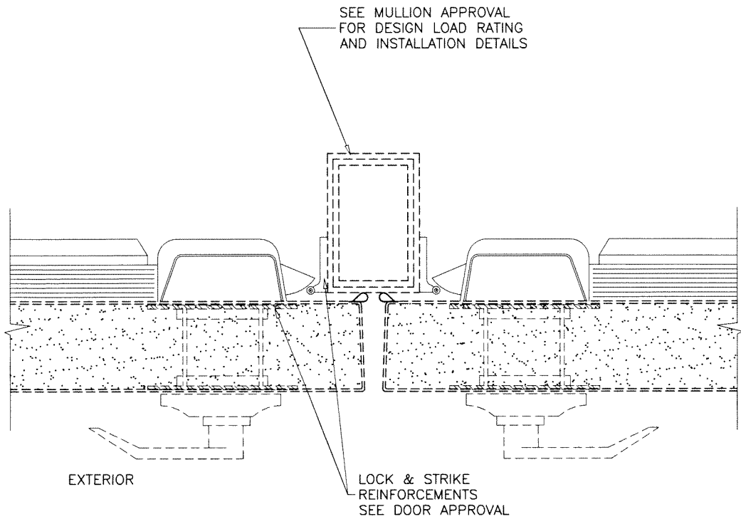
SECTION D-D '6200' SERIES RIM EXIT DEVICE WITH SERIES 9200 MULLION
