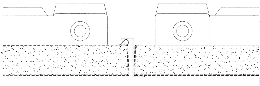
SECTION F-F '6200' SERIES SVR EXIT DEVICE
